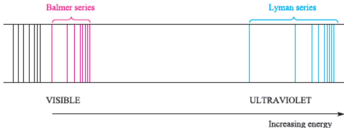
Figure 4. Spectrum of hydrogen
