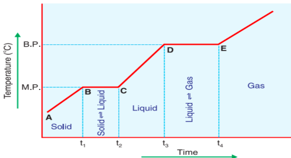
Figure 3.5 Heating curve.
