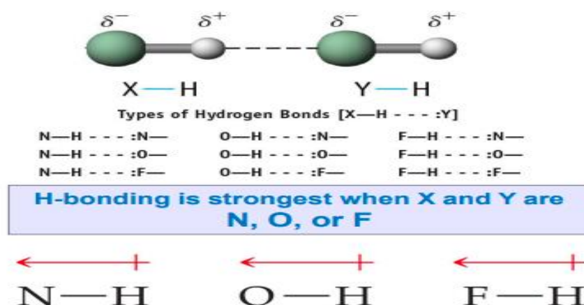
Figure 3.4 hydrogen bonding
