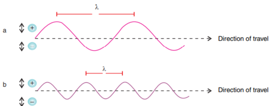
Figure 5. Electromagnetic wave
