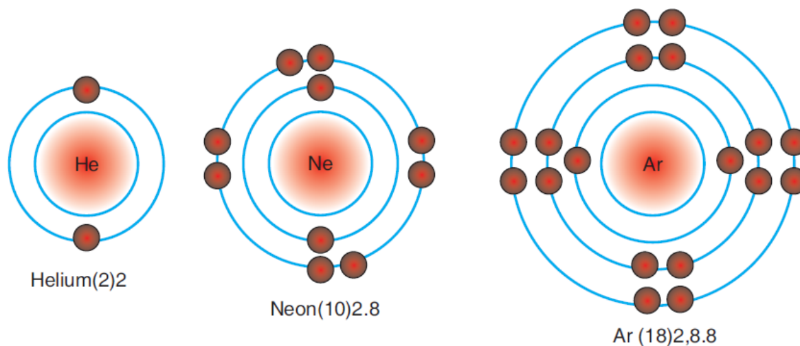
Figure 1. First three noble gases.
