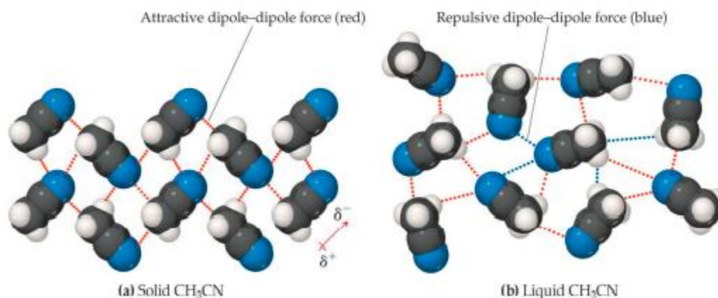
Figure 3.3 dipole forces
