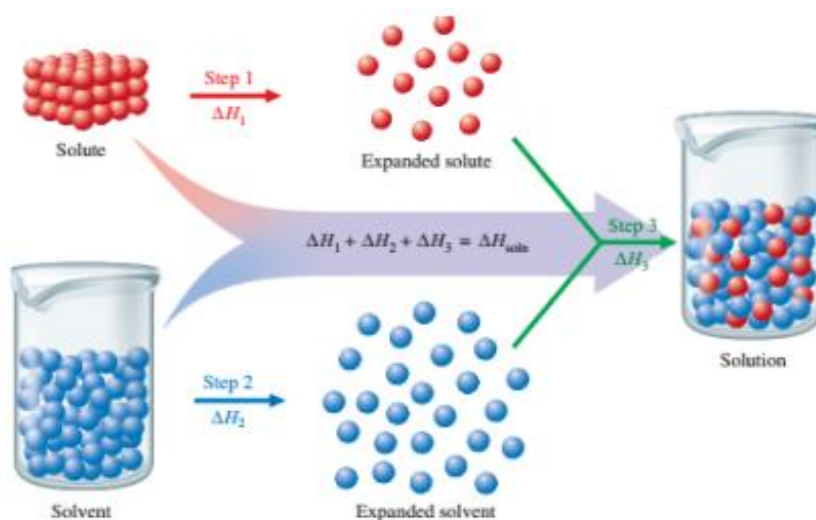
Figure 4.1 A molecular view of the solution process, portrayed as taking place in three steps
